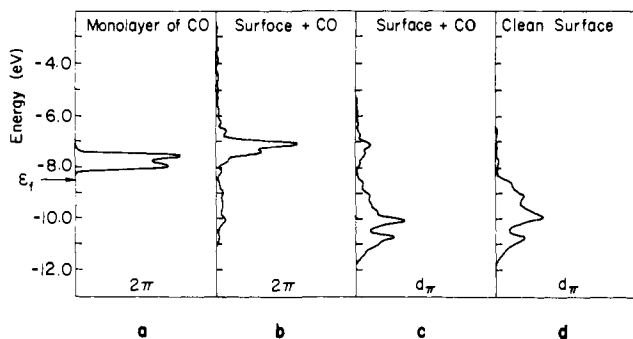
Figure 7. Projected DOS for (a) 2\pi of a monolayer of CO, (b) 2\pi of the same CO, adsorbed, (c) d_\pi levels of those surface atoms having adsorbed CO, and (d) d_\pi of the clean metal surface.
