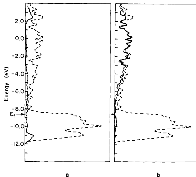
Figure 2. Projected DOS of a Ni(100) four-layer slab. The solid line indicates s states in part a and p states in part b. The broken lines are the total DOS in both parts a and b. The peak between -8 and -12 eV indicates mainly d states penetrated by s and p states.
