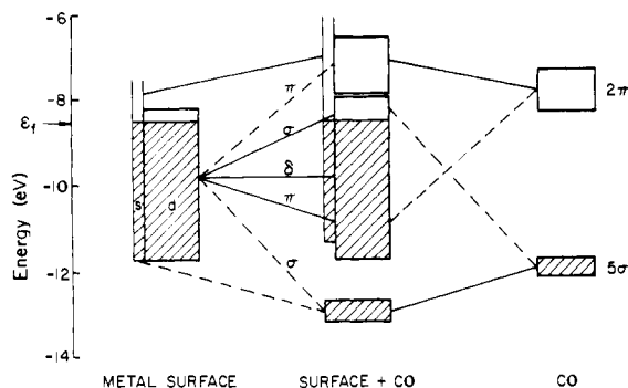
Figure 9. Principal interactions in the c(2 \times 2)\text{CO-Ni}(100) chemisorption system. The solid lines indicate major contributions while dashed lines point to weaker mixing. The open bars are meant to indicate that there is a substantial number of states at still higher energy.
