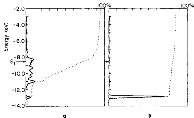
Figure 6. Projected DOS of (a) d_x of those surface atoms which have CO adsorbed on them and (b) 5\sigma of CO in the c(2 \times 2) CO-Ni(100) system. The dotted line is an integration. Those states above the Fermi level in part b illustrate the electron density decrease from 2 to 1.62 (see Table I).
