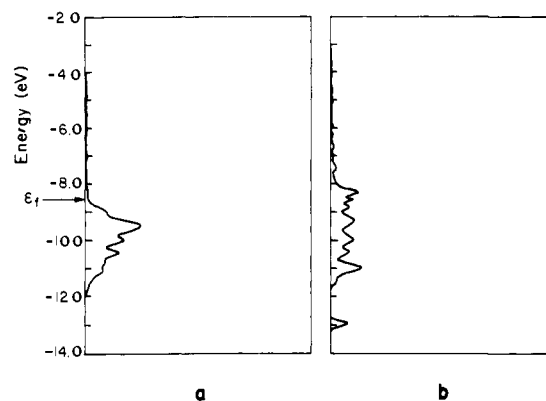
Figure 5. Projected DOS of d_{z^2} of (a) a clean surface layer and (b) those surface atoms having adsorbed CO. The increase of DOS above the Fermi level in part b, compared to that in part a, corresponds to the 0.50 electron density decrease in d_{z^2} (see Table I).
