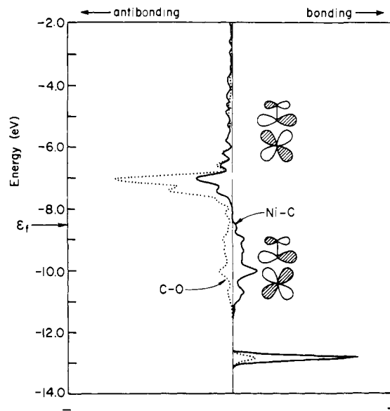
Figure 8. Crystal orbital overlap population in the c(2 \times 2)\text{CO-Ni}(100) chemisorption system.
