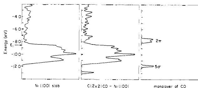
Figure 4. Total DOS of a Ni(100) slab, a c(2 \times 2) CO-Ni(100) system, and a monolayer of CO.
