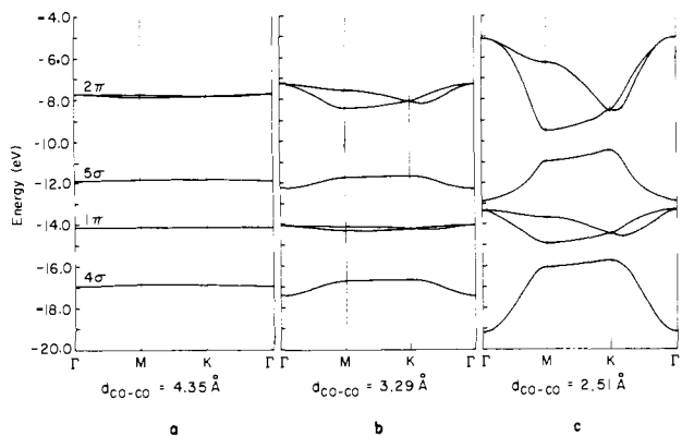
Figure 1. Band structures of monolayer CO along the symmetry lines indicated by \Gamma M , MK , and K\Gamma for CO-CO distances 4.35, 3.29 and 2.51 Å.
