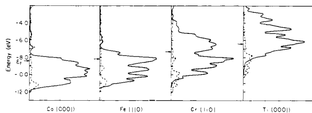
Figure 10. Calculated DOS of the surface layer of Co, Fe, Cr, and Ti four-layer slabs. Solid lines are the projected d states and broken lines the projected s states; the arrow indicates the Fermi level.
