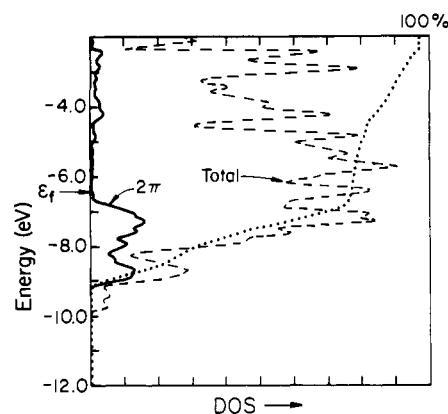
Figure 11. Projected DOS of 2 \pi of CO on the Ti(0001) surface. The dotted line is the integrated DOS of 2 \pi . The broken line is the total DOS of the chemisorption system.
