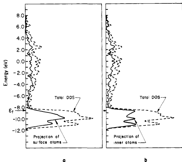
Figure 3. Projected DOS of surface and inner layers of a Ni(100) four-layer slab. In better, self-consistent calculations similar dispersing effects are observed, but the surface states are more skewed toward the Fermi level.
